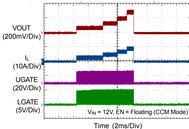
Power On in Short Circuit
