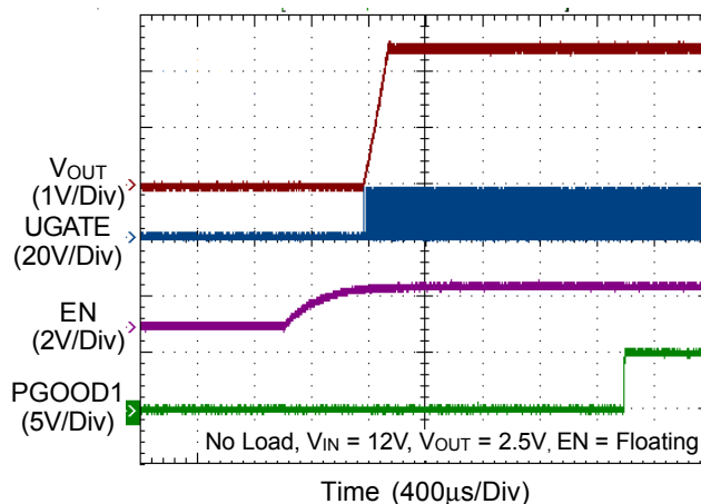
Power On from EN (CCM Mode)
