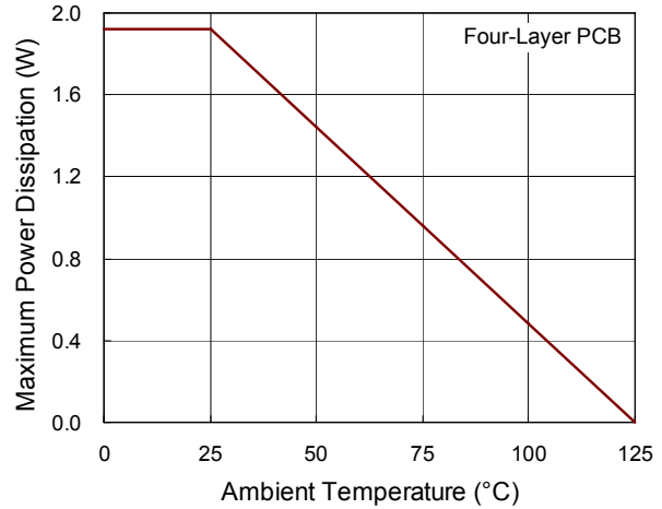
Figure 7. Derating Curve for the RT8205L/M Package
