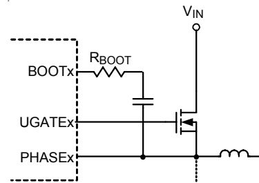
Figure 4. Reducing the UGATEx Rise Time
