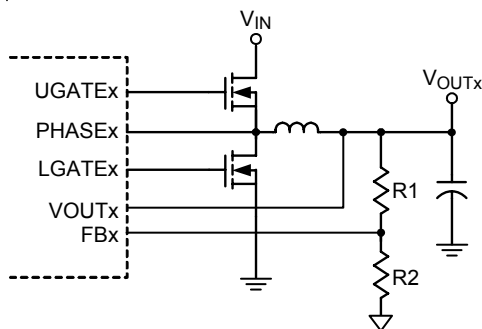
Figure 6. Setting V OUTx with resistor divider
