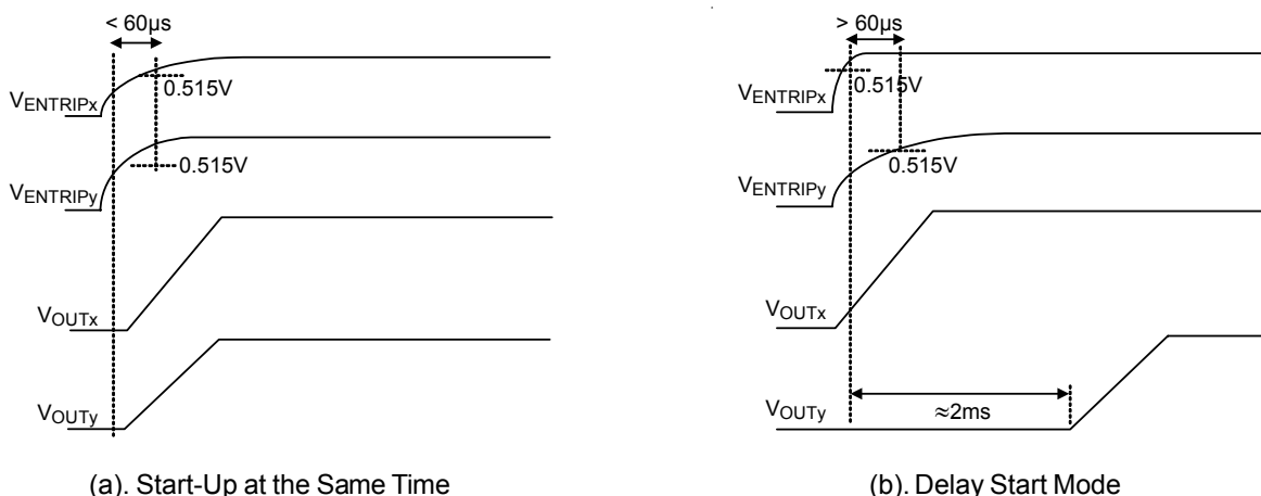
Figure 5. Time Diagrams of Power Sequence
