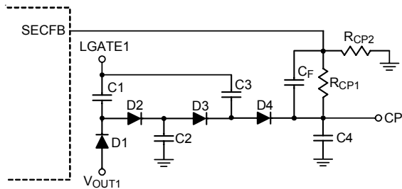
Figure 3. Charge Pump Circuit Connected to SECFB
